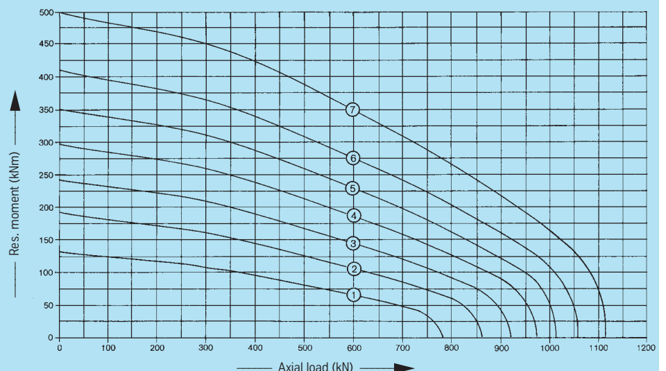
Service life curves · 30,000 revolutions
