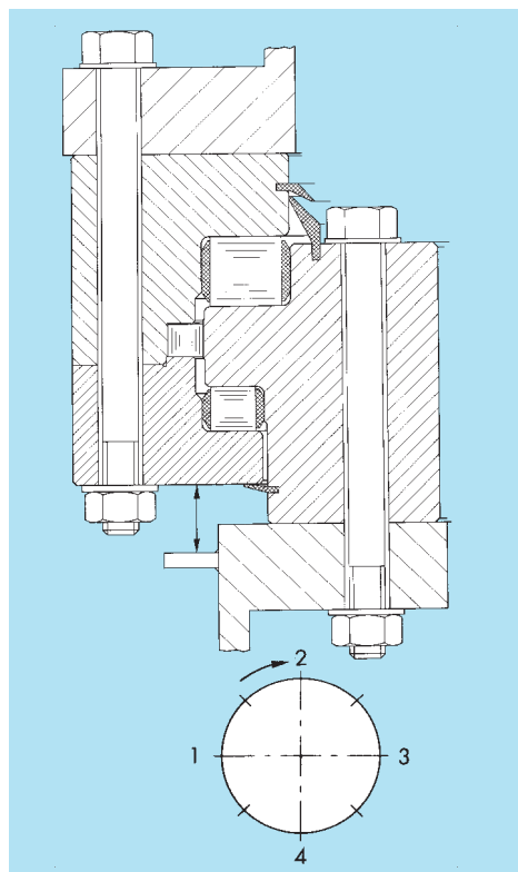
Fig. 35: Three-row roller slewing bearing ring – basic test setup for axial reduction measurement
