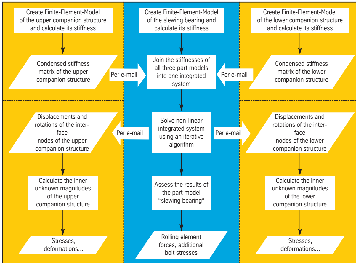
Schematic of the calculation method designed by Rothe Erde (Fig. 5)
