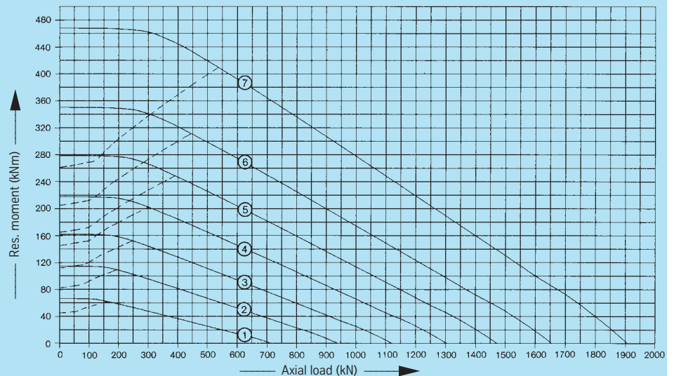
Static limiting load curves
