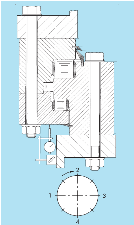
Fig. 32: Three-row roller bearing slewing ring – basic test setup for tilting clearance measurement
