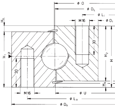
Drawing number 060.22.0575.502.11.1504
