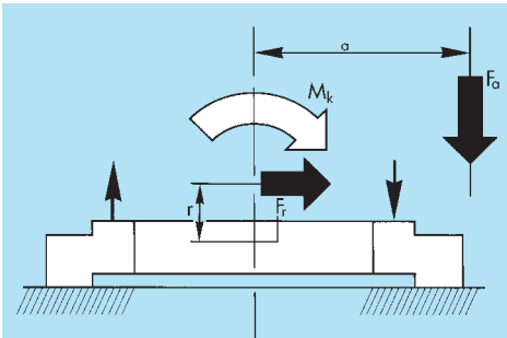
Fig. 31: Loading principle for tilting clearance measurement
