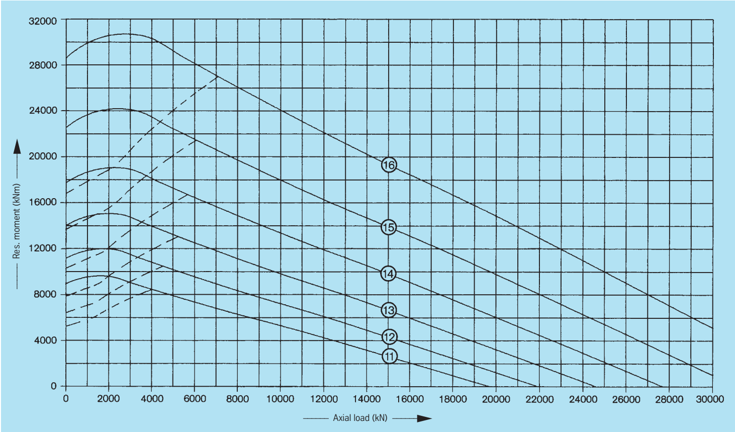
Static limiting load curves ——— Raceway — — — Bolts Bearing rings quenched and tempered
