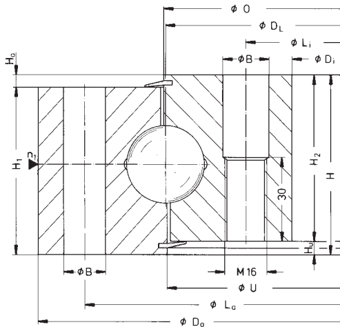
Drawing number 060.22.0370.301.11.1504 060.22.0505.000.11.1503 060.22.0660.001.11.1503
